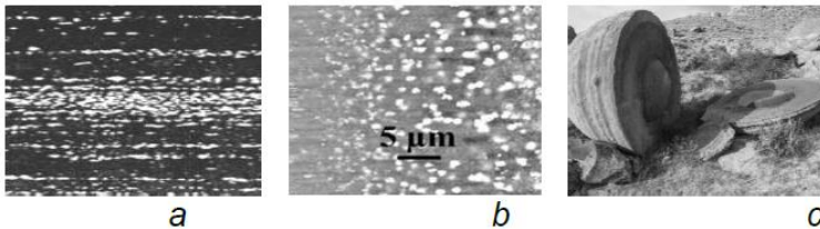
Fig. 1. Non-homogeneous structures of damask steel with sorbitol matrix and the accumulation of secondary cementite (a) [6], silicon with spherical nickel inclusions (b) [10] and rock formations (c) [14]
