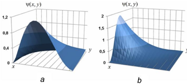
Fig. 2. Correlation function \psi(x, y)
