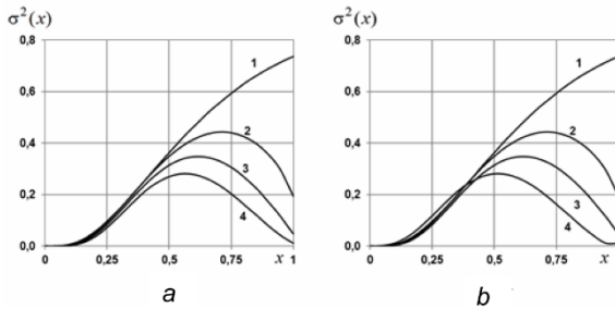
Fig. 3. Dispersion \sigma^2(x)
