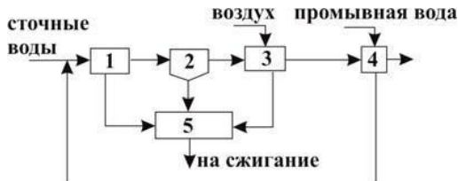
Fig. 1. Typical scheme of wastewater treatment from petroleum products at thermal power plants:
