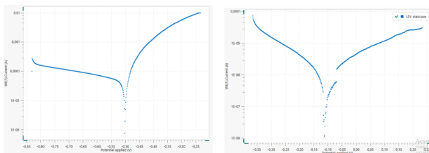
Figure 1. Polarization curves of electrospark coatings: a - sample No. 1; b- sample No. 5.
